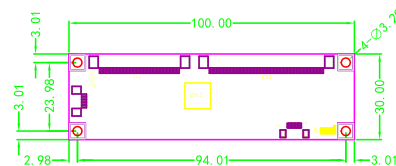
SCALE(1:3) ILITEK 2312 Controller
